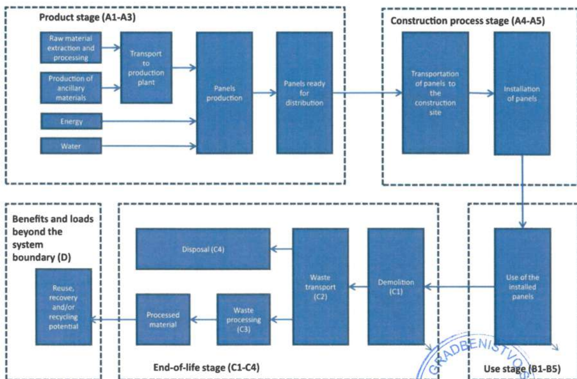
Figure 1: Schematic representation of the system boundaries
